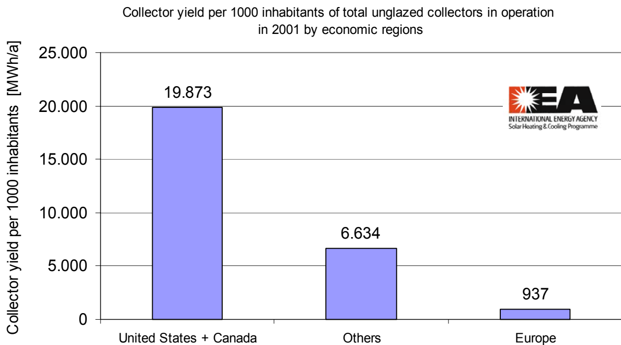
Figure 16: Annual collector yield of unglazed collectors in operation by economic region in the year 2001
